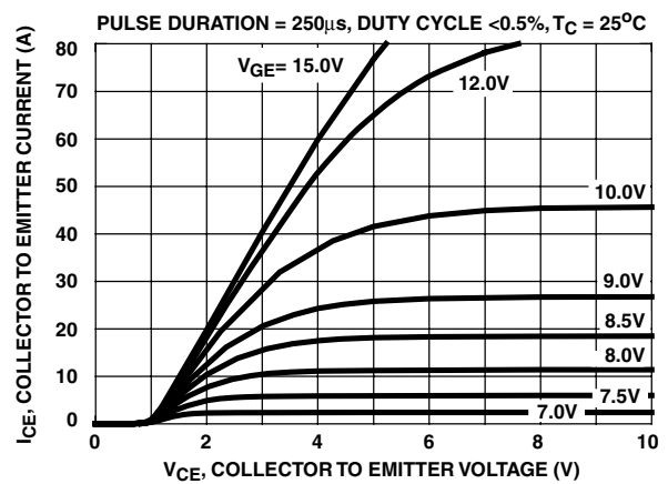
FIGURE 2. SATURATION CHARACTERISTICS
