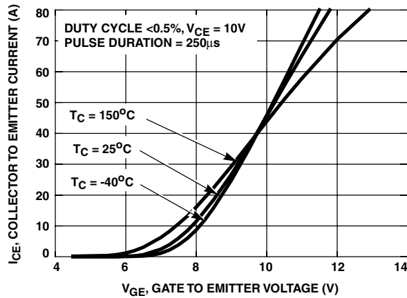
FIGURE 1. TRANSFER CHARACTERISTICS
