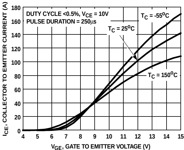
FIGURE 13. TRANSFER CHARACTERISTIC
