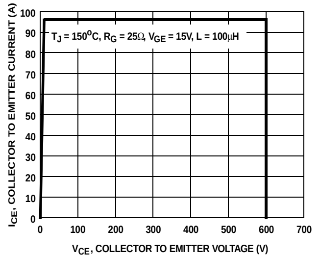
FIGURE 2. MINIMUM SWITCHING SAFE OPERATING AREA
